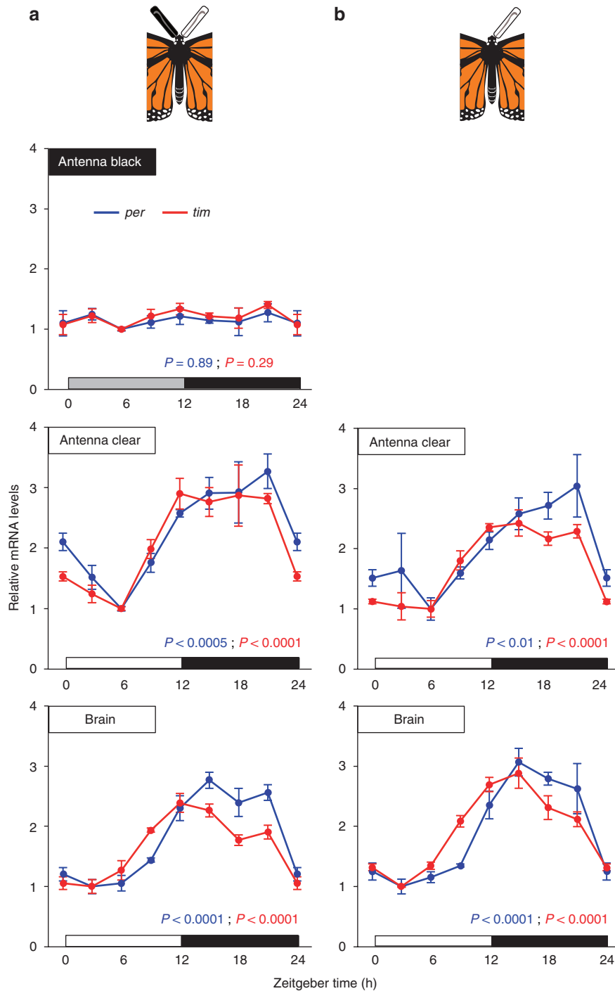
Figure 3 | Molecular correlates of circadian timing in the antennae and brain. (a) Antenna and brain profiles of per and tim expression in migrants with a clear- and black-painted antenna. Top, experimental condition for collections. Values are relative to the minimal level for each gene and are mean \pm s.e.m. of three antennae or three brains. Points at ZT 0 are re-plotted at ZT 24 to show the 24-h trend. Horizontal bars show the light cycle: open, lights on; grey, lights on in black-painted antenna; black, lights-off. P -values, one-way analysis of variance. (b) Antenna and brain profiles of per and tim expression in migrants in which the black-painted antenna was removed. Top, experimental condition for collections.
